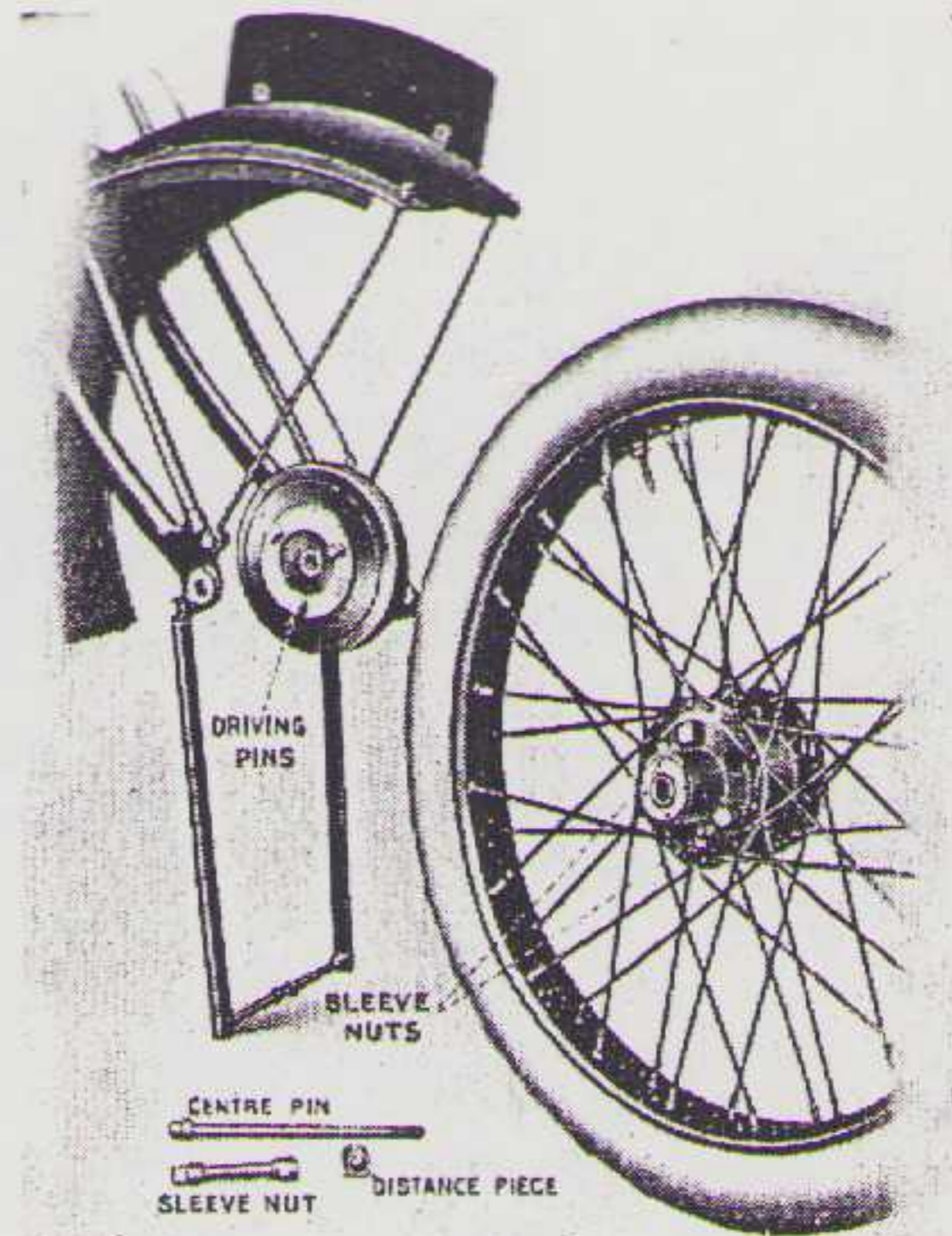
Showing Front Wheel detached and its interchangeability with Rear Wheel.
