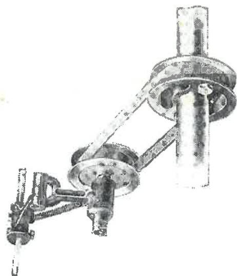
Figure 10. Type No. AA181. The Smith Cardan Shaft Drive.
