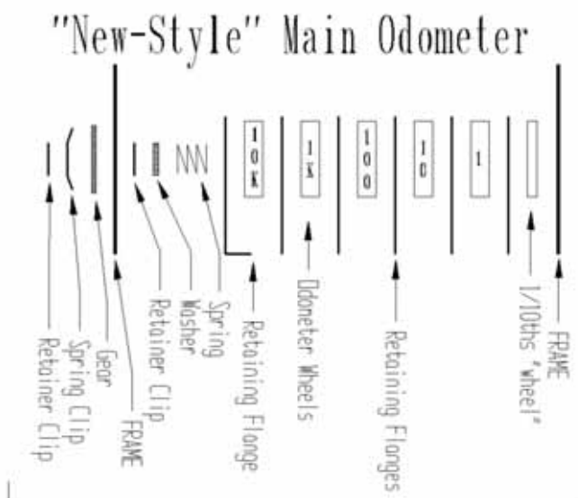
Figure 8. Diagram of "new-style" odometer components
